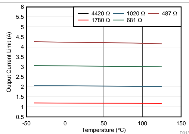
Figure 12. OVC Threshold vs Temperature
