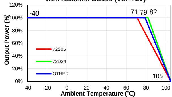
EC7BW18-72 Derating Curve with Heatsink BC100 (Vin=72V)
