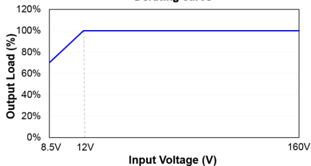
EC7BW18-72 Input Voltage Derating Curve
