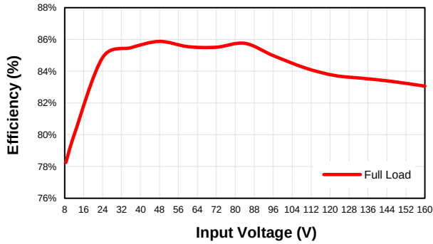
EC7BW18-72S05 Eff Vs Vin @25 Deg. C
