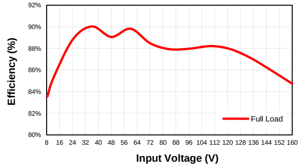
EC7BW18-72S12 Eff Vs Vin @25 Deg. C
