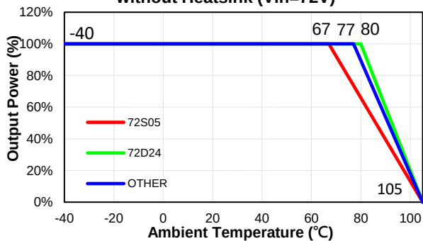
EC7BW18-72 Derating Curve without Heatsink (Vin=72V)
