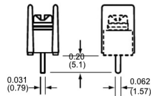
02 Printed Circuit
