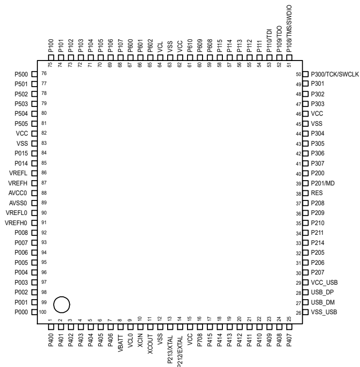
Figure 1.4 Pin assignment for LQFP 100-pin
