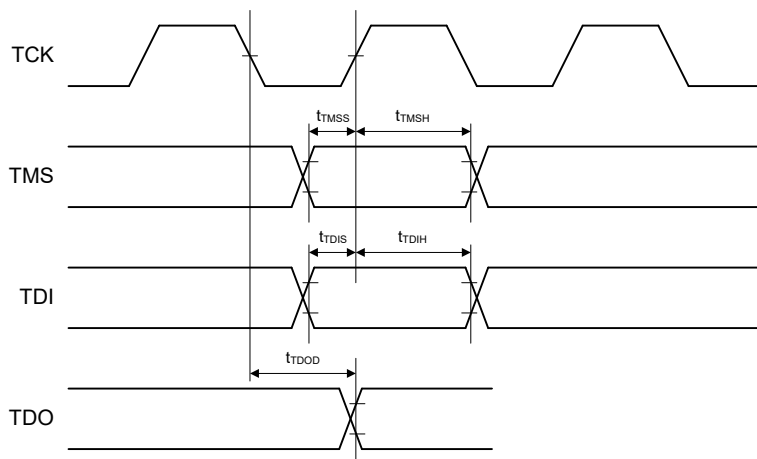
Figure 2.64 Boundary scan input/output timing
