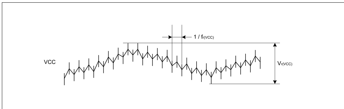
Figure 2.6 Ripple waveform
