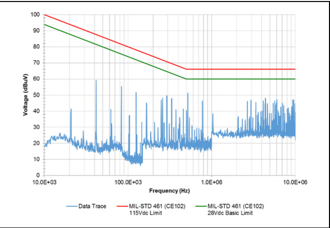
HQA2W120W280V-007-S typical Conducted Emissions with FQB filter module and 0.01 \mu F common mode capacitors.
