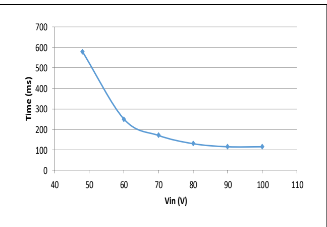
FQB typical input over-voltage shutdown envelope.
