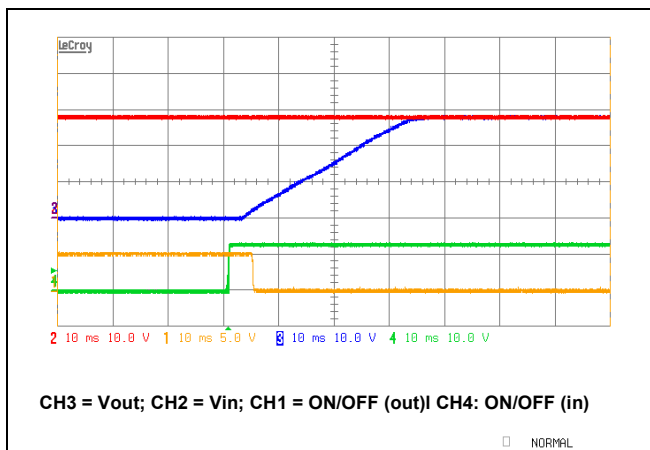
FQB typical startup from Input ON/OFF signal application, I_o = 0.5A .
