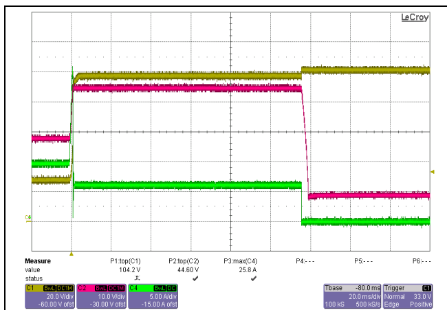
FQB typical response to 28V to 100V input voltage step, Time = 20 ms/div, CH1 = Vin (20V/div), CH2 = Vo (10V/div).
