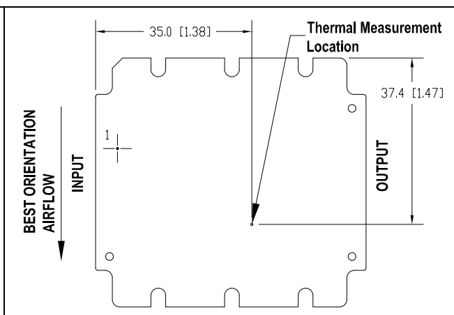
FQB020ADC thermal measurement location – top view.
