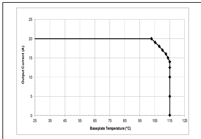
FQB020ADC maximum output current vs. baseplate temperature.
