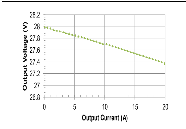
FQB typical Load Regulation characteristics.
