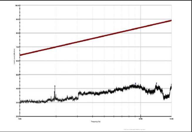
MIL-STD-461 Method RE102 Typical High Frequency Radiated Emissions.
