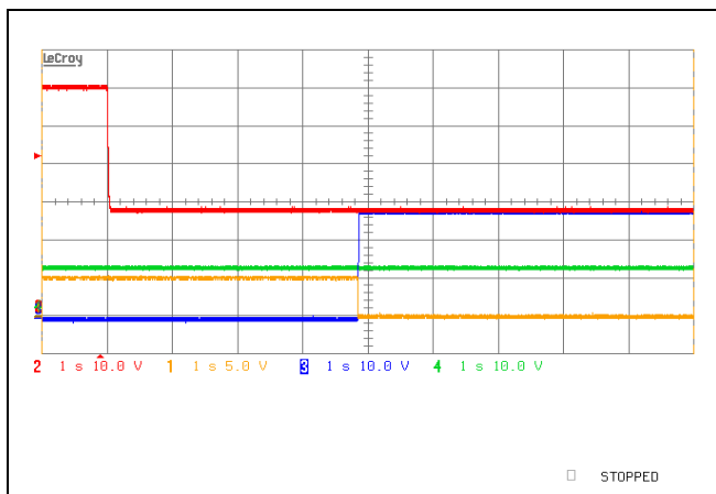
FQB typical auto-recovery response during 60V to 28V input voltage recovery, time = 1s/div.
