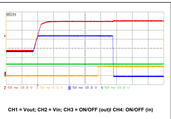
FQB typical response to 28V to 60V input voltage step, Time = 50 ms/div.
