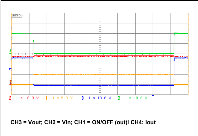
FQB typical response to severe overload event at output, (1s/div)
