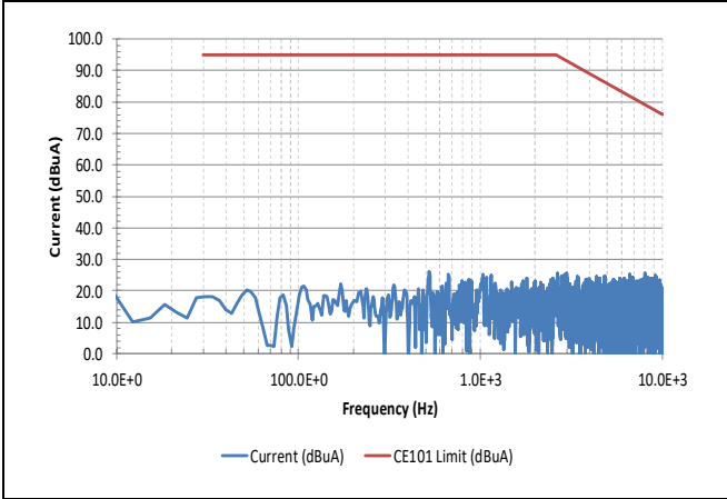
MIL-STD-461G Method CE101 Typical Low Frequency Conducted Emissions.
