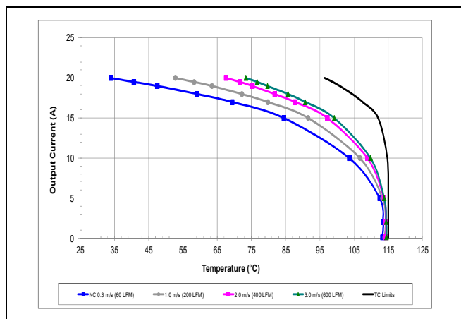
Maximum output current vs. ambient temperature at nominal input voltage for natural convection (60lfm) to 600lfm with airflow from pin 1 to pin 3.
