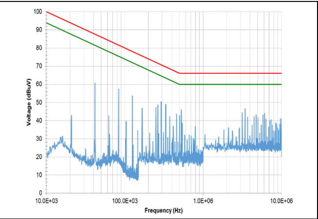
HQA2W120W050V-007-S typical Conducted Emissions with FQB filter module and 0.01 \mu F common mode capacitors.
