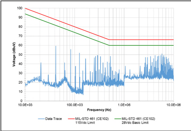
HQA24120W480V-007-S typical Conducted Emissions with FQB filter module and 0.01 \mu F common mode capacitors.
