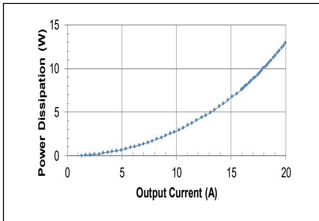
FQB typical Power Loss characteristics.
