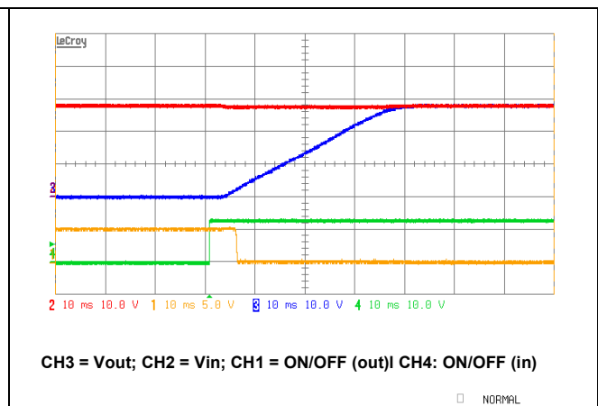
FQB typical startup from Input ON/OFF signal application with 5,000 \mu F electrolytic capacitor load; I_o = 0.5A .
