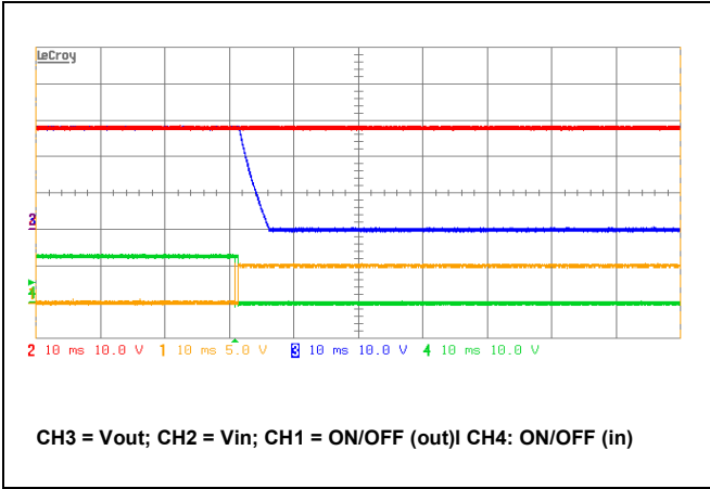
FQB typical shut down from Input ON/OFF signal application, I o = 0.5A.
