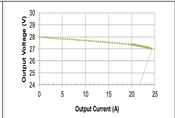
FQB typical Current Limiting characteristics.
