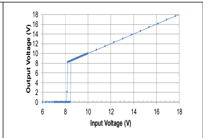
FQB typical Input Voltage vs. Output Voltage characteristics.
