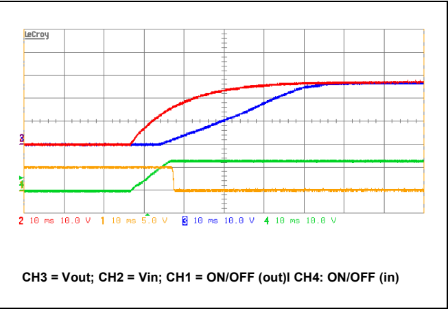
FQB typical startup from Input Voltage application, R load = 1.4Ω = 20A at 28V.
