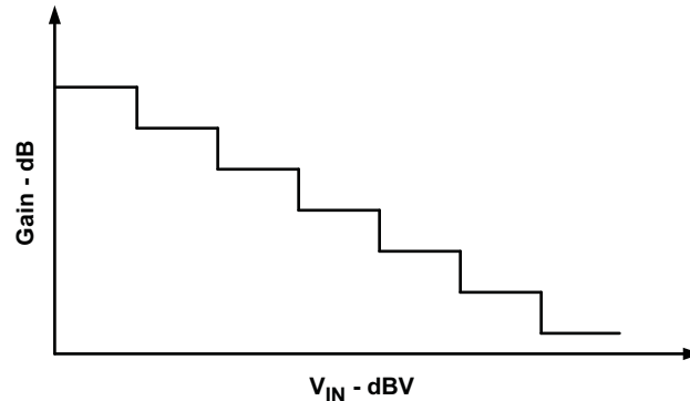
Figure 33. Input Signal Voltage vs Gain
