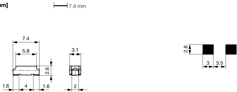
Soldering pads
