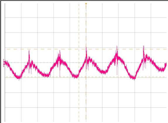
Figure 1: ADH700-48S50-6LS Input reflected Ripple Current Waveform Ch1 : Iin (2uS/div, 10mA/div)
