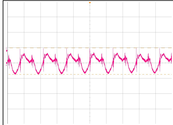
Figure 2: ADH700-48S50-6LS Ripple and Noise Measurement Ch1 : Vo (5uS/div, 50mV/div)
