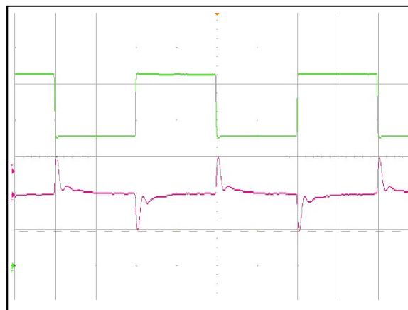
Figure 8: ADH700-48S50-6LS Transient Response (50mS/div) 25% load step(50%~75%~50%), 0.1A/us slew rate Ch 4: Vo (500mV/div) Ch 2: Io (2A/div)
