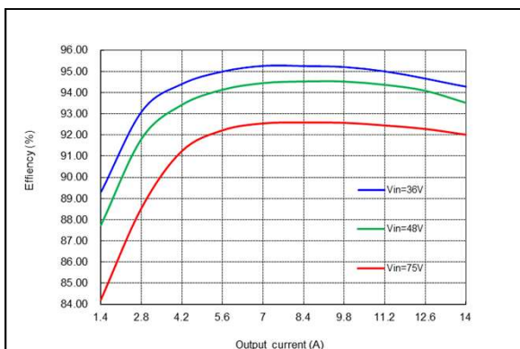
Figure 9: ADH700-48S50-6LS Efficiency Curves @ 25 °C, 400LFM, Vo=50V Loading: Io = 10% increment to 14A
