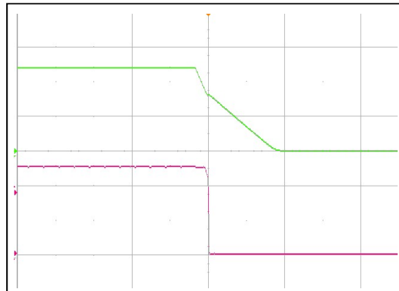
Figure 4: ADH700-48S50-6LS Output voltage shut down by power Off (50ms/div) Ch 2: Vin (20V/div) Ch 4: Vo (10V/div)
