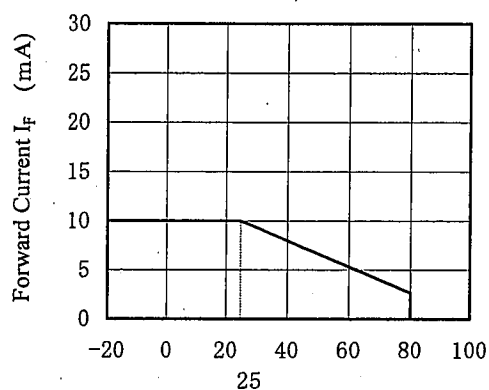
Case Temperature T_c (°C) Forward Current Derating Curve
