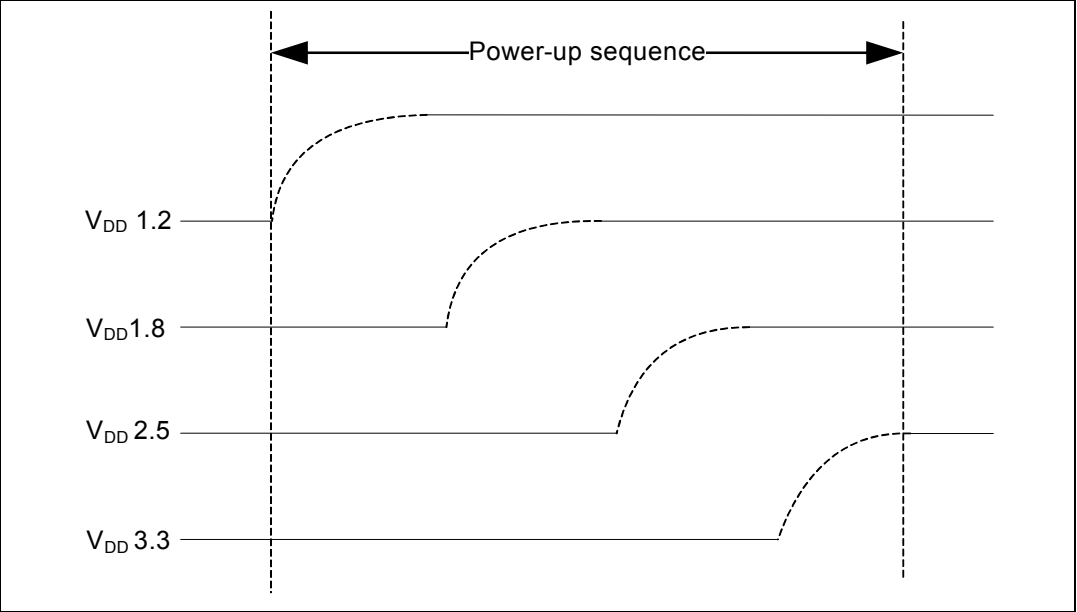
Figure 6. Power-up sequence
