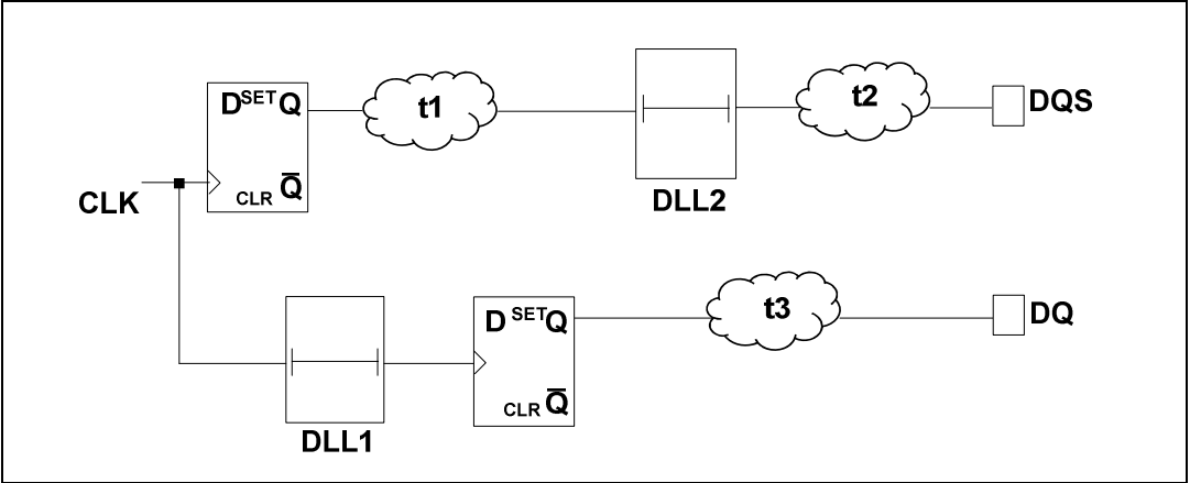
Figure 11. DDR2 Write cycle path
