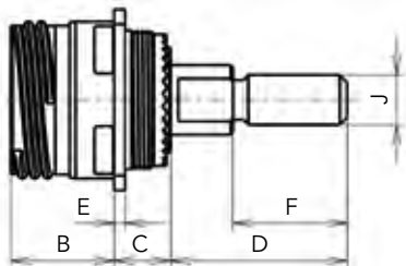
With 8D0 (square flange receptacle)
