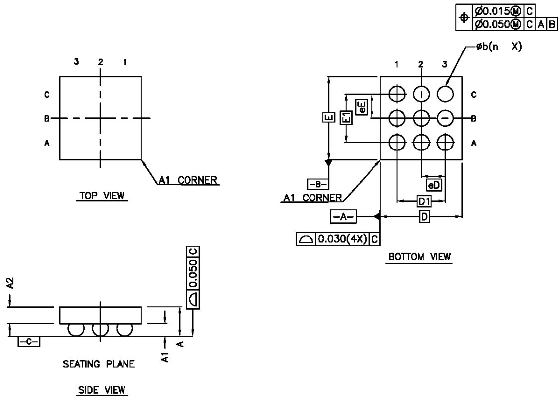
Figure 6. 9-ball CSP Package Outline
