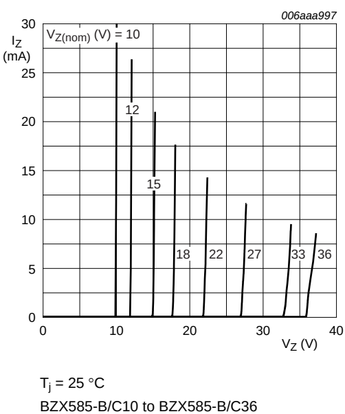
Fig 6. Working current as a function of working voltage; typical values
