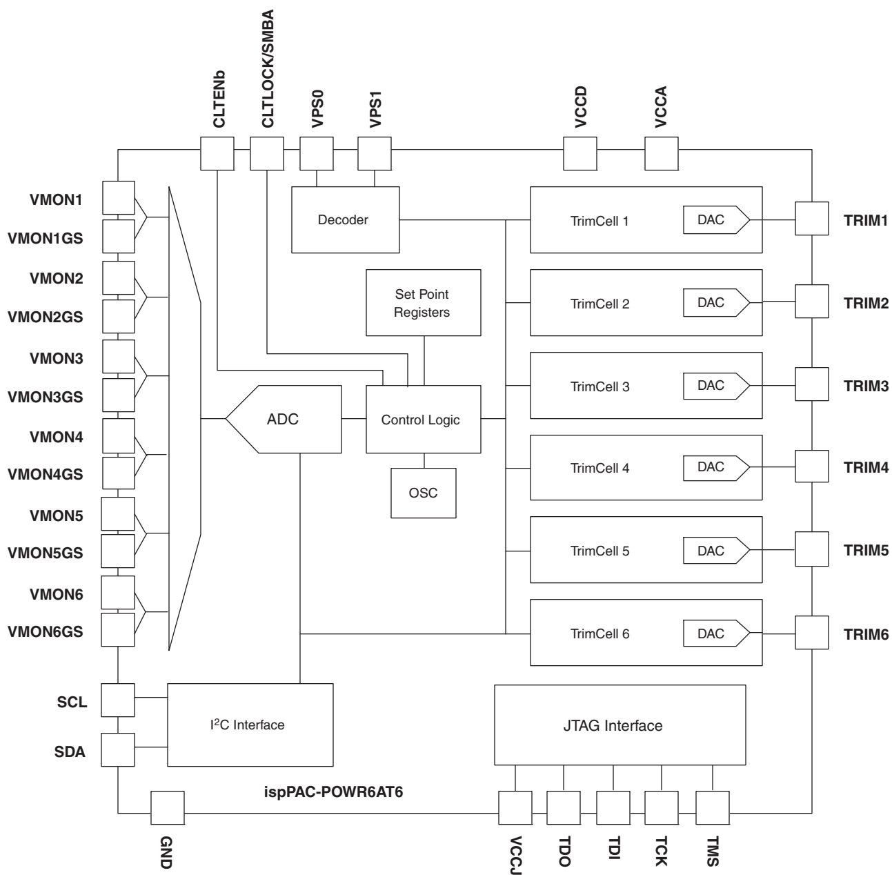
Figure 3-1. ispPAC-POWR6AT6 Block Diagram
