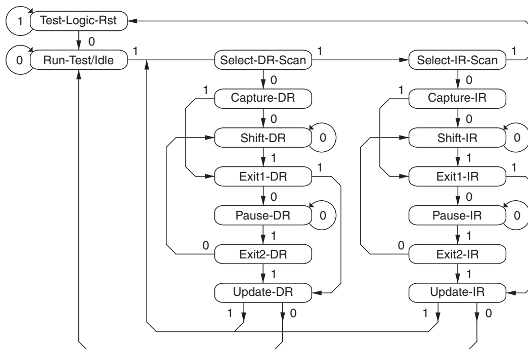
Figure 3-26. TAP States
