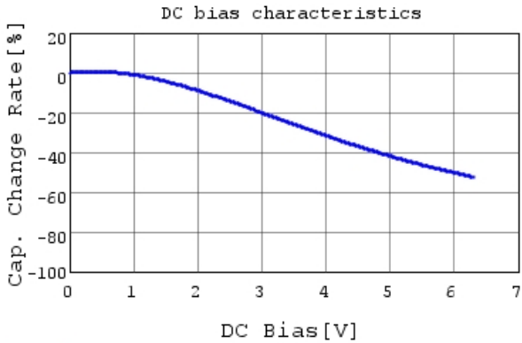
GCJ188C70J335KE02 C-DC bias capchange, 25.0c
