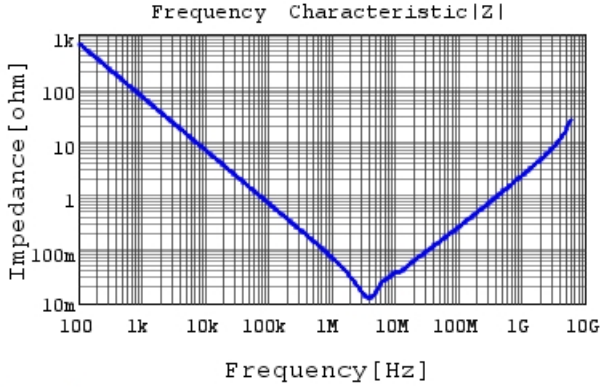
GCJ188C70J335KE02 |Z| DCOV, 25degC
