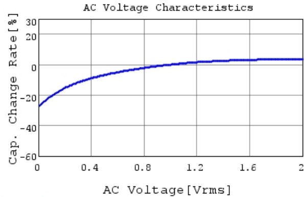
GCJ188C70J335KE02 C-AC Voltage capchange, Dc
