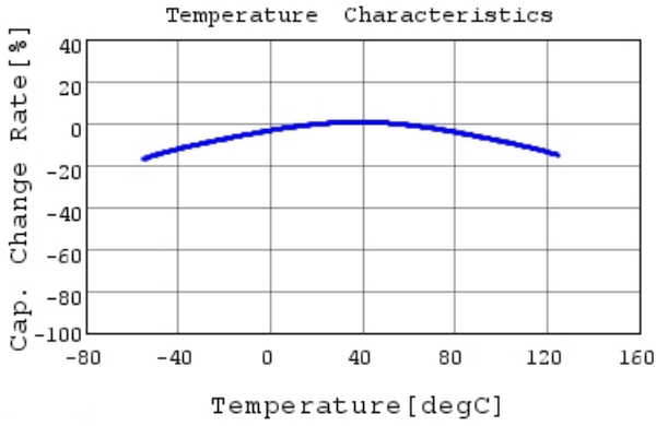
GCJ188C70J335KE02 C-Temp. capchange, DC0.0V,
