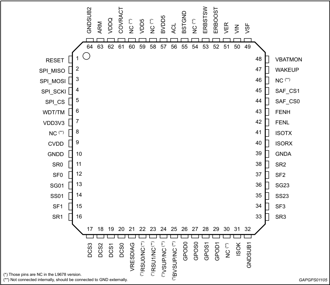
Figure 1. Pin-out description
