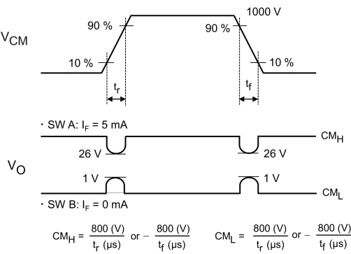
Fig. 13.1.8 Common-Mode Transient Immunity Test Circuit and Waveform
