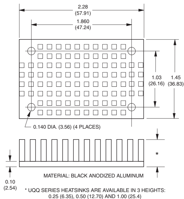
Figure 8. Optional Heatsink
