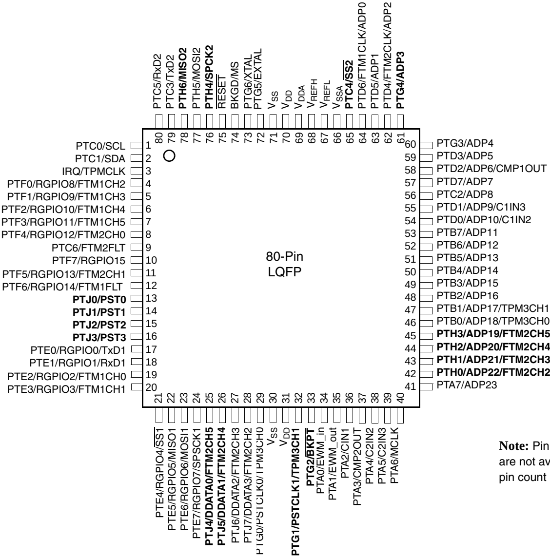
Figure 2. 80-Pin LQFP
