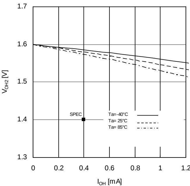
Figure 10. Output High Voltage2 vs Output Current (Vcc=1.6V)
