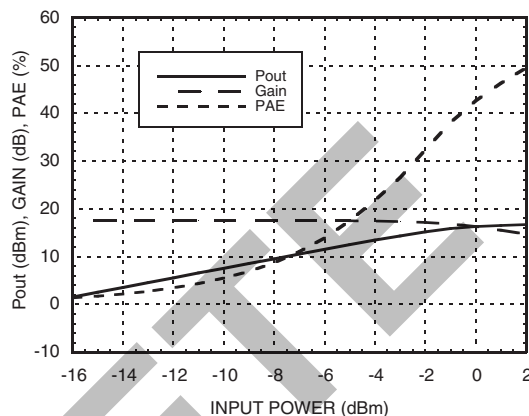
Power Compression @ 900 MHz [1]
