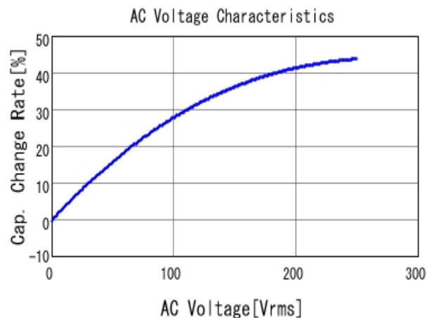
■ DE2E3KY102MN3AM02F C-AC Voltage capchange, DCOV, 20.0
