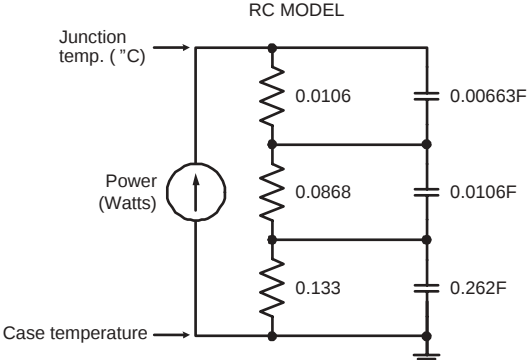
FIGURE 19B, TRANSIENT THERMAL IMPEDANCE MODEL
