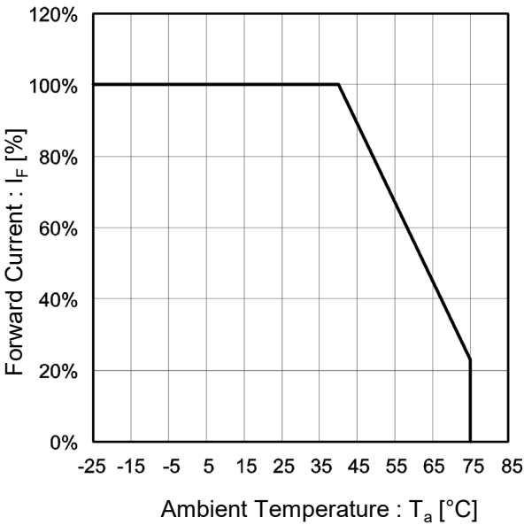
Fig.6 Derating
