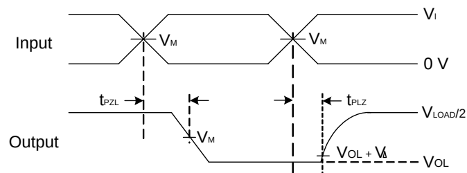
Voltage Waveforms Inverting and Non Inverting Outputs
