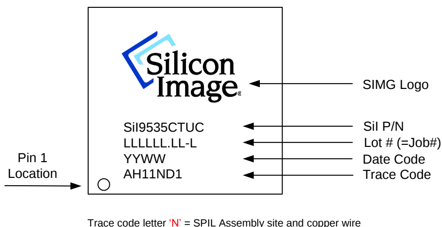
Figure 8.2. Marking Diagram
