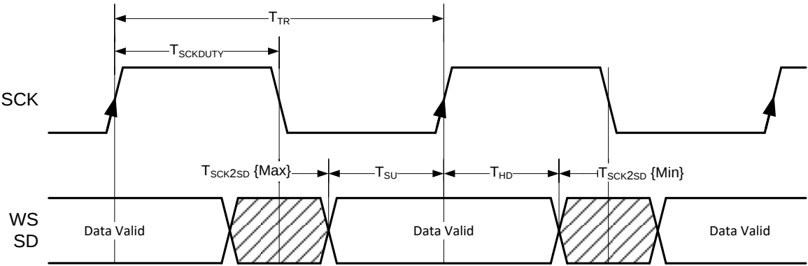
Figure 4.6. I²S Output Timing
