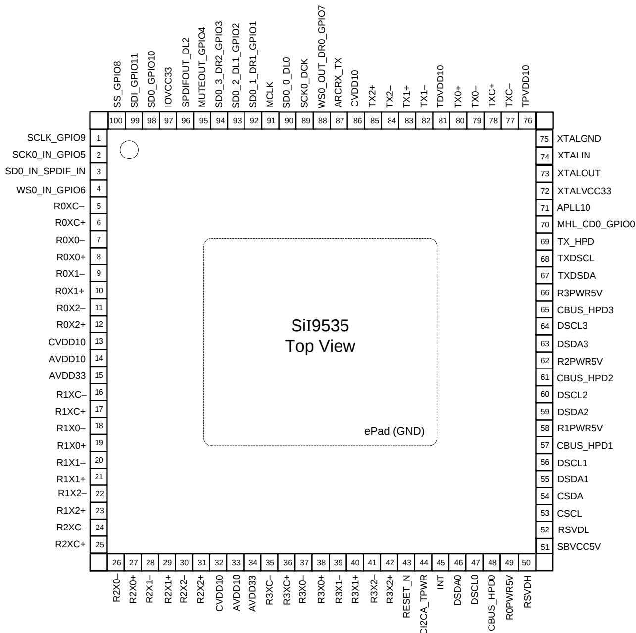
Figure 5.1. Pin Diagram
