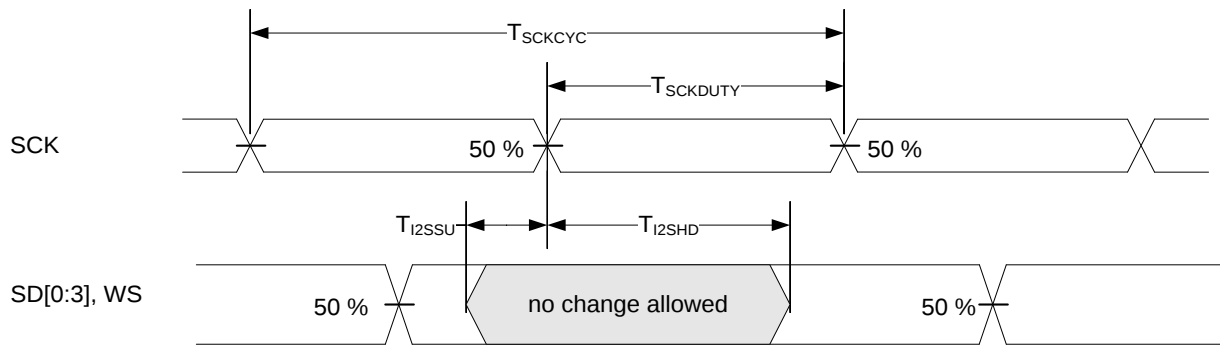
Figure 4.4. I²S Input Timing
