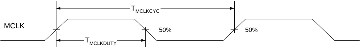
Figure 4.8. MCLK Timing
