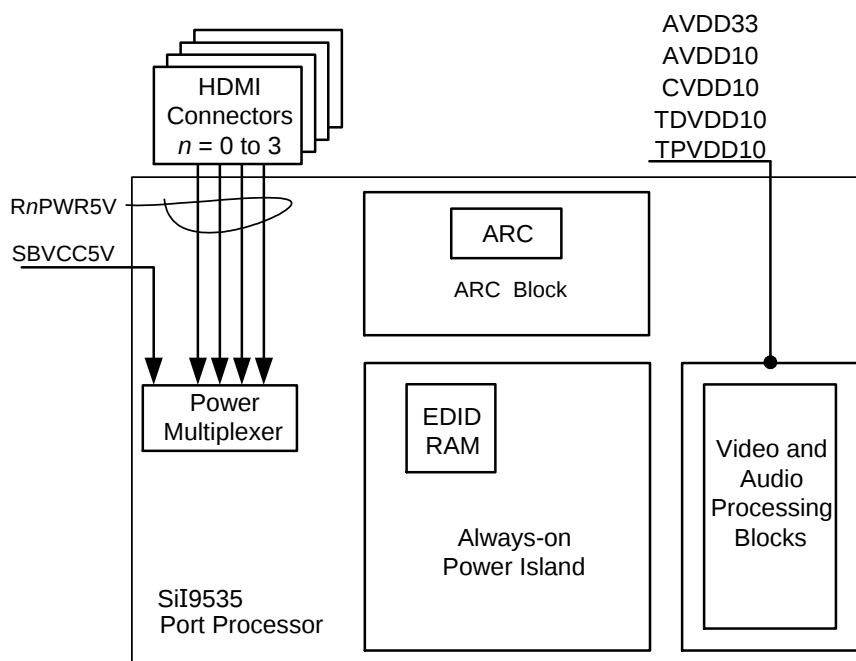
Figure 6.1. Standby Power Supply Diagram
