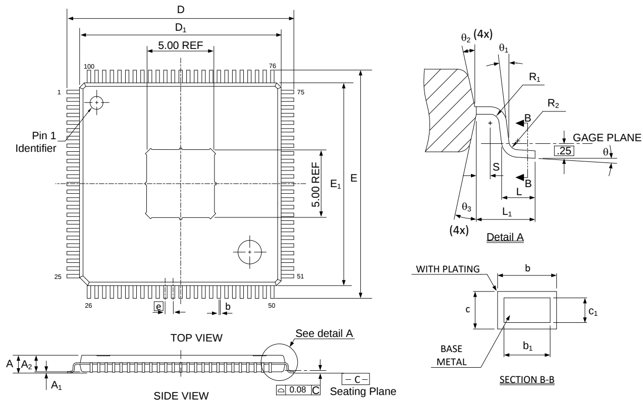
Figure 8.1. Package Diagram
