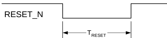
Figure 4.2. RESET_N Minimum Timing
