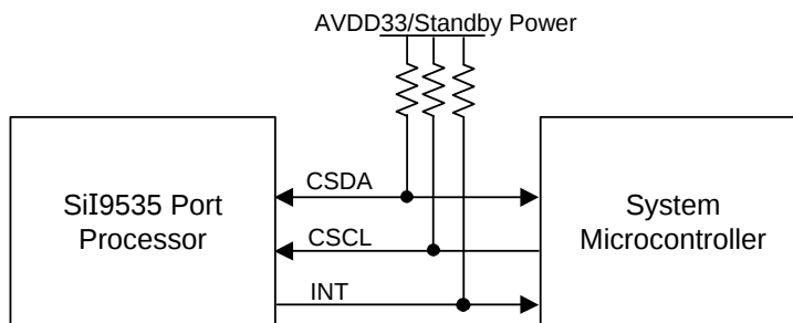
Figure 2.2. I 2 C Control Mode Configuration
