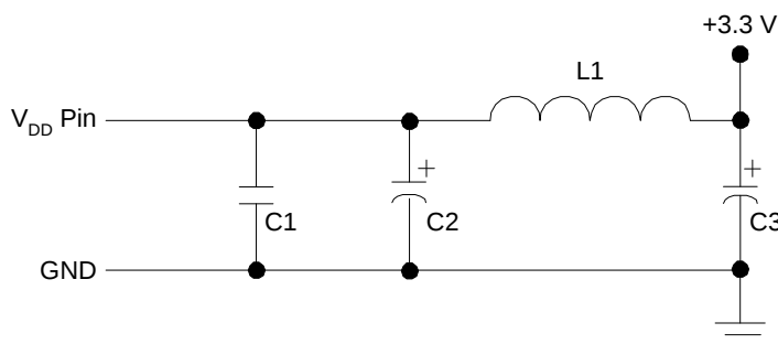
Figure 7.1. Decoupling and Bypass Schematic Diagram
