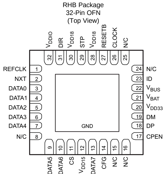
Pin Functions
