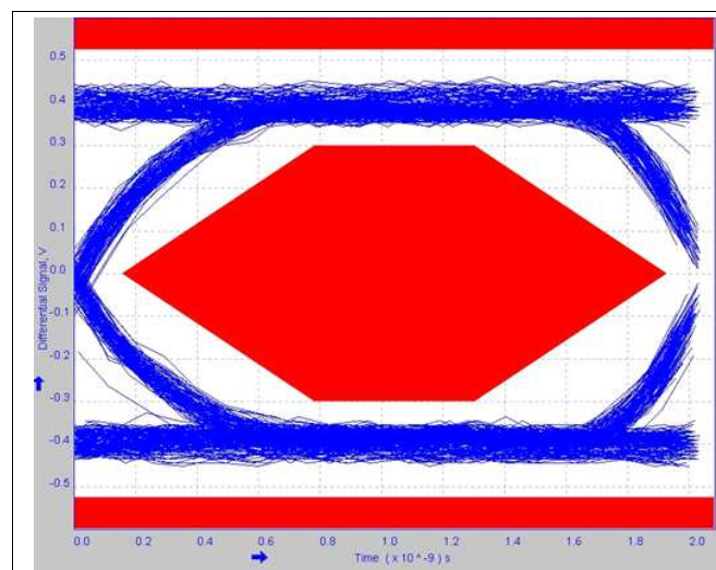
Figure 4-2. High-Speed Eye Diagram
