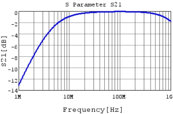
DE1B3KX471KN4AP01F S21 DCOV, 20degC
