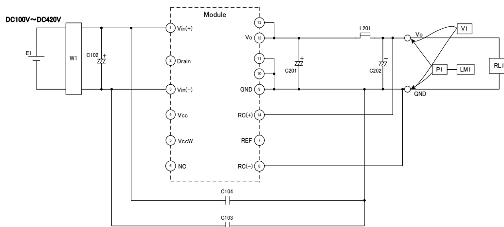
Measurement circuit
