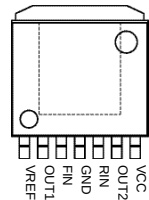
Figure 4. HRP7 (TOP VIEW)
