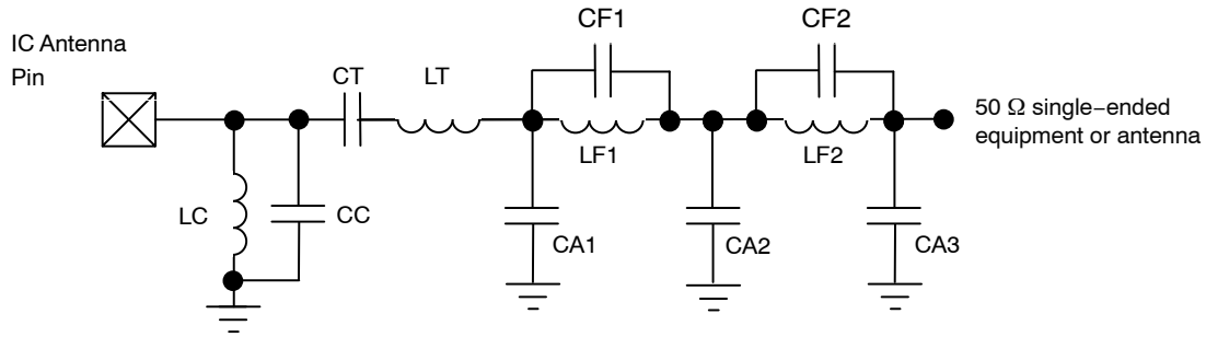
Figure 9. Structure of the Single-ended Antenna Interface for TX Operation to 50 \Omega Single-ended Equipment or Antenna
