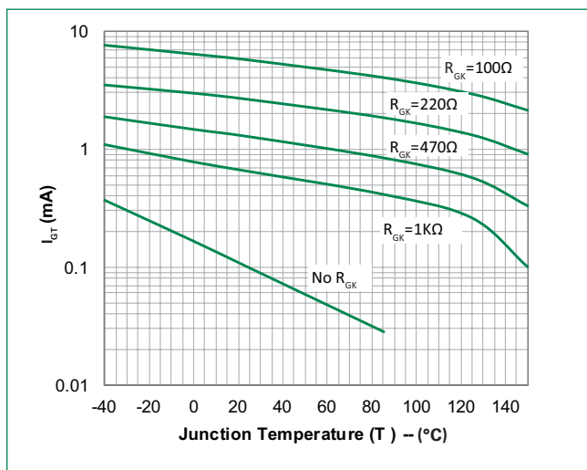
Figure 11: Typical DC Gate Trigger Current with R_{GK} vs. Junction Temperature (Sensitive SCR)
