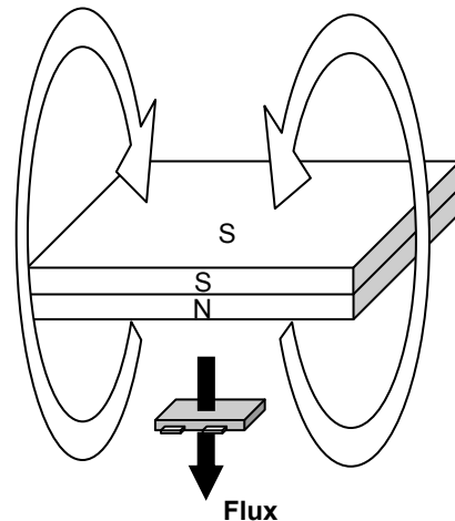
Vertically Stacked Magnet
