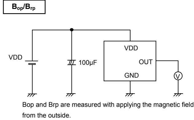
Fig.1 B_{op}, B_{rp} measurement circuit
