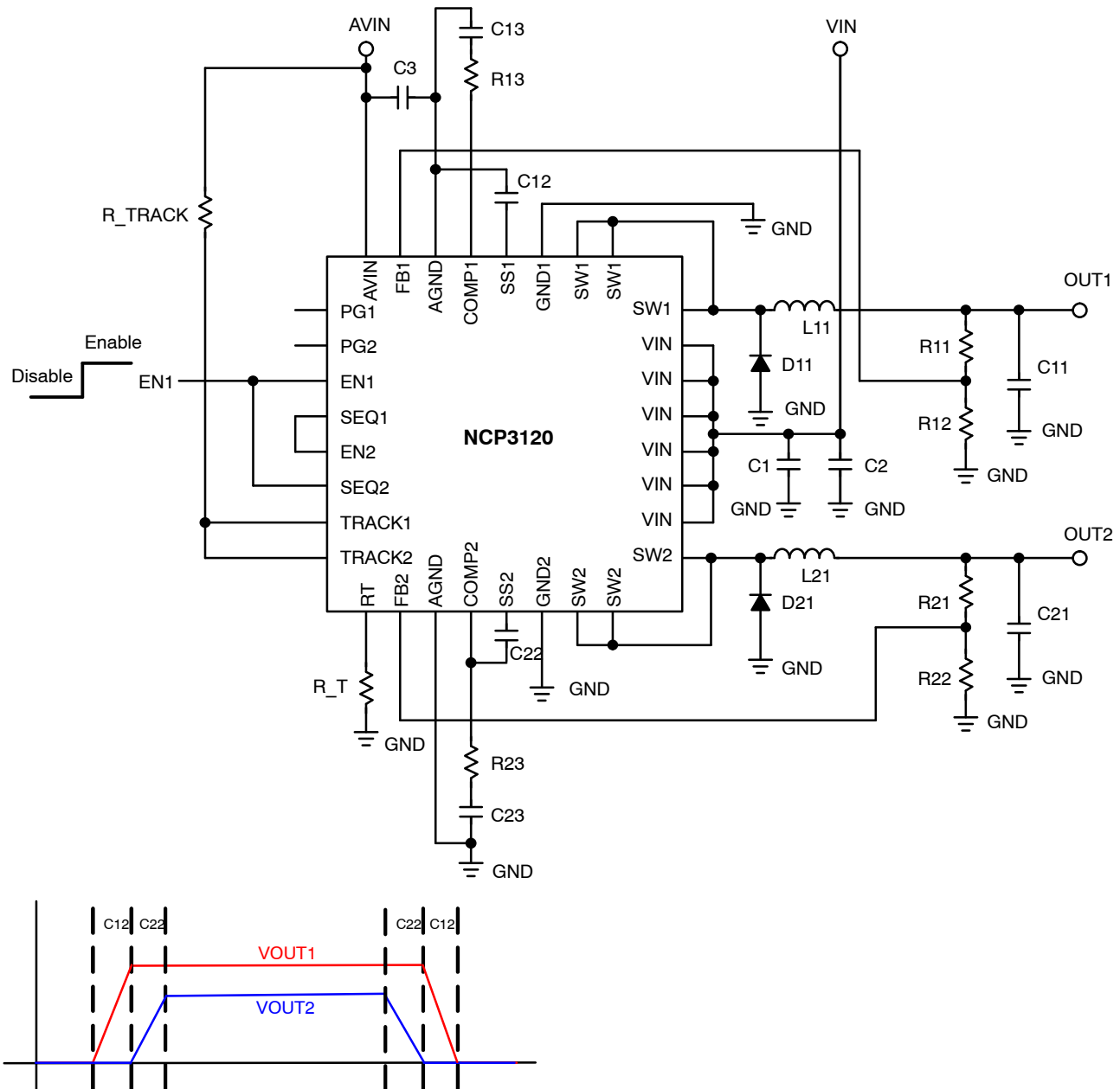
Figure 43. Sequential Configuration
