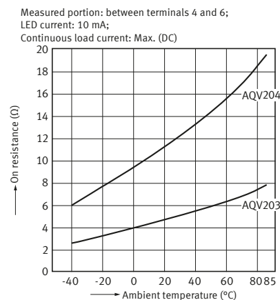
2-4. On resistance vs. ambient temperature characteristics ( AC/DC type: AQV203, AQV204 )
