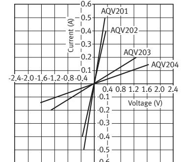
7-2. Current vs. voltage characteristics of output at MOS portion ( AC/DC type )
