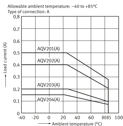
1-2. Load current vs. ambient temperature characteristics ( AC/DC type )
