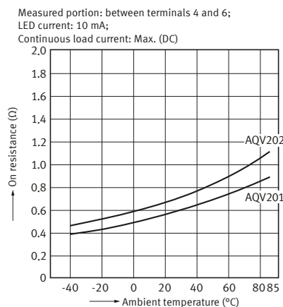
2-3. On resistance vs. ambient temperature characteristics ( AC/DC type: AQV201, AQV202 )
