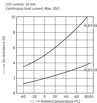
2-2. On resistance vs. ambient temperature characteristics ( DC type: AQV103, AQV104 )
