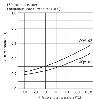
2-1. On resistance vs. ambient temperature characteristics ( DC type: AQV101, AQV102 )
