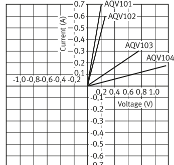
7-1. Current vs. voltage characteristics of output at MOS portion ( DC type )
