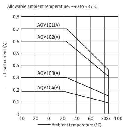
1-1. Load current vs. ambient temperature characteristics ( DC type )
