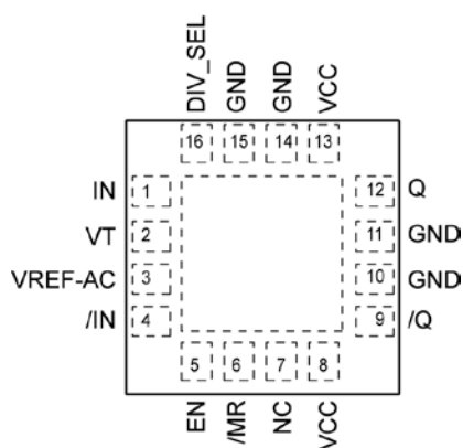
16-Pin QFN
