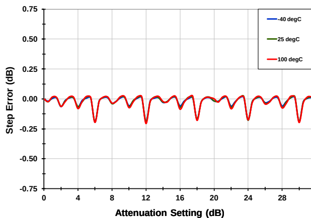
DNL [900 MHz]
