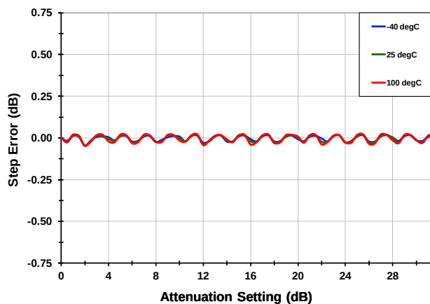
DNL [1900 MHz]
