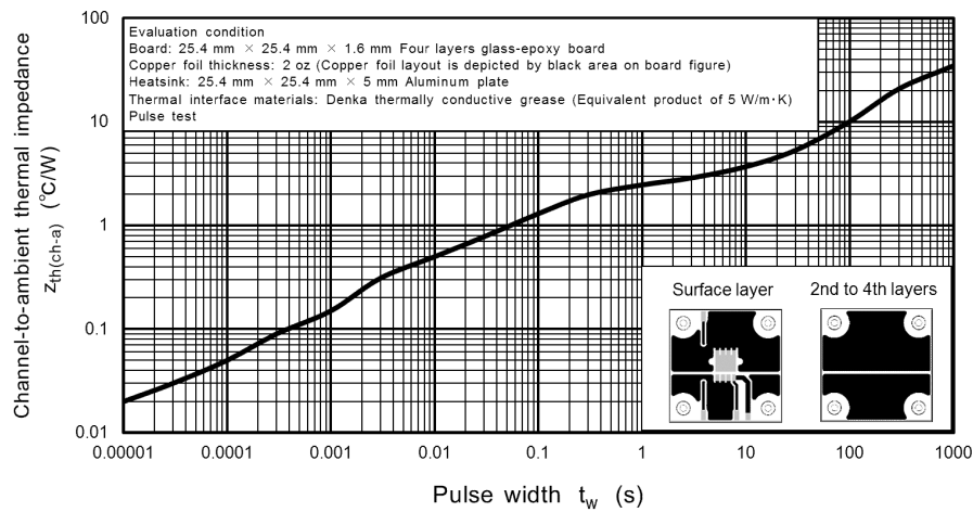
Fig. 8.18 Z_{th(ch-a)} - t_w (Reference Values)
