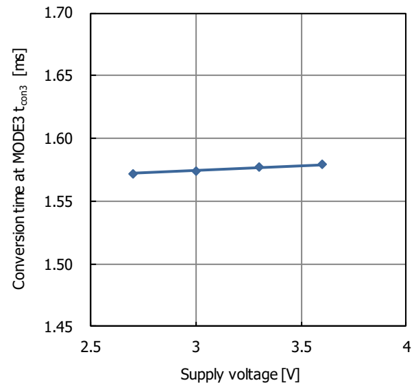
Fig. 19.10 Conversion time at MODE 3 supply voltage characteristic
