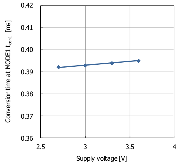
Fig. 19.6 Conversion time at MODE 1 supply voltage characteristic
