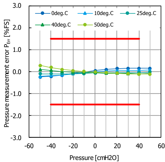
Fig. 20.3 Pressure measurement error P_{Err} temperature characteristic 0~50deg.C
