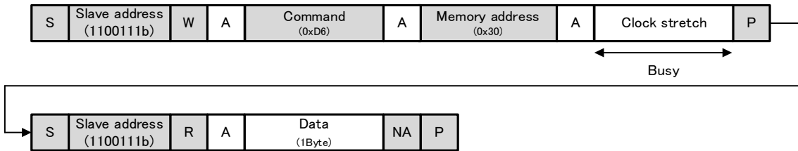
Fig. 17 I2C NVM Read format
