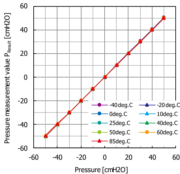
Fig. 20.1 Pressure measurement value P_{Result} temperature characteristic
