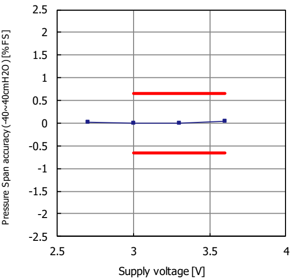
Fig. 20.7 Pressure Span accuracy P_{Sacc} supply voltage characteristic
