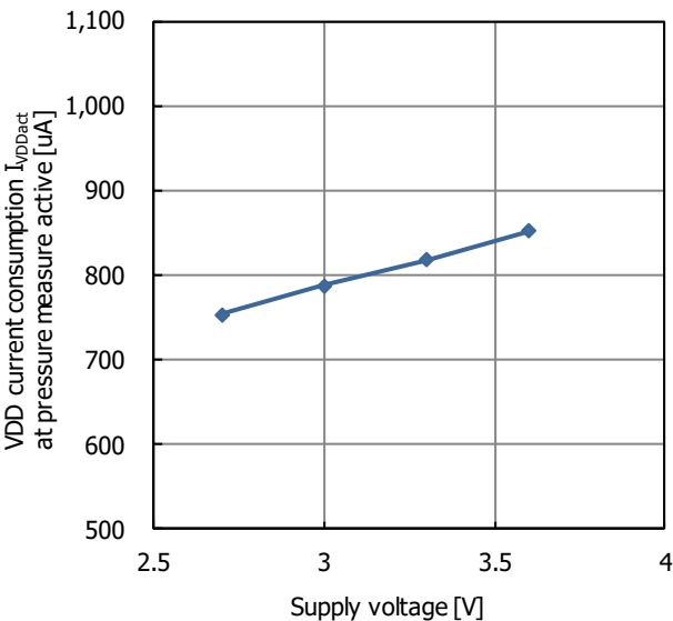
Fig. 19.2 VDD current consumption I_{VDDact} at pressure measure active supply voltage characteristic
