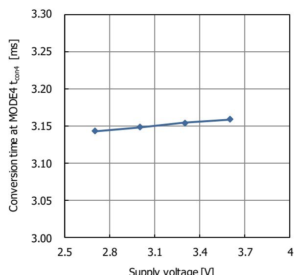
Fig. 19.12 Conversion time at MODE 4 supply voltage characteristic
