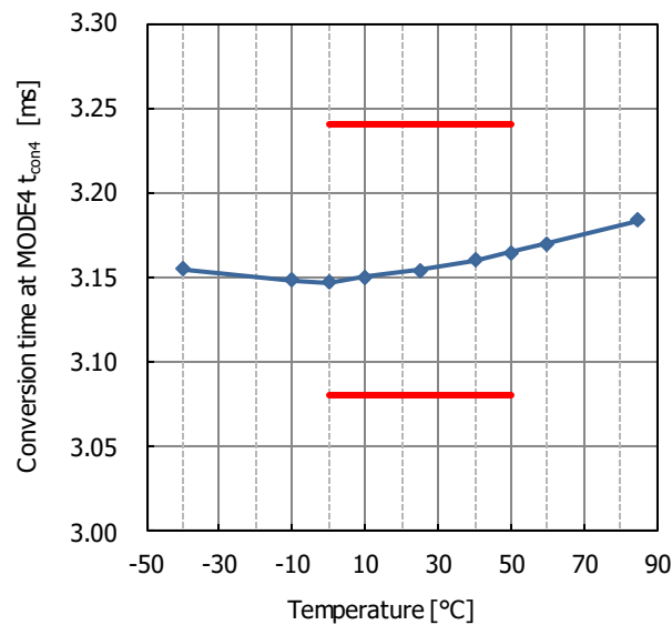
Fig. 19.11 Conversion time at MODE 4 temperature characteristic
