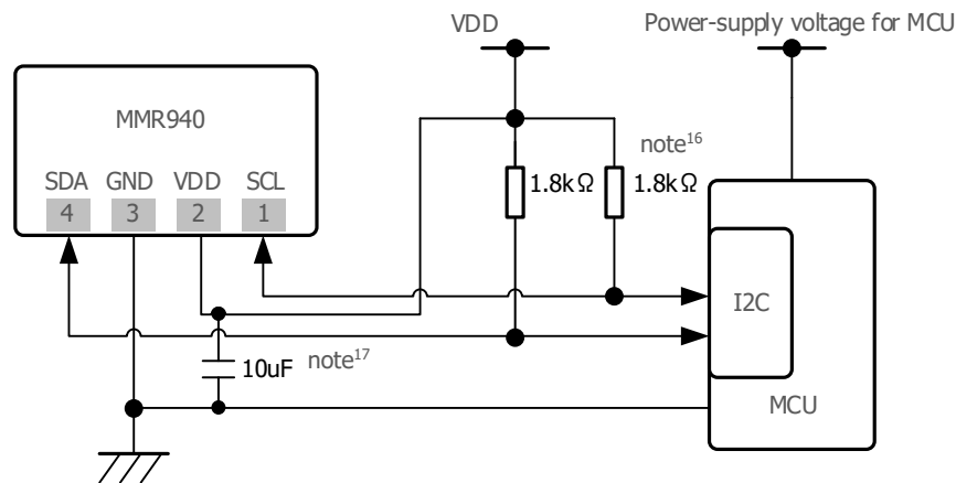
Fig. 18 Typical Electrical Connection
