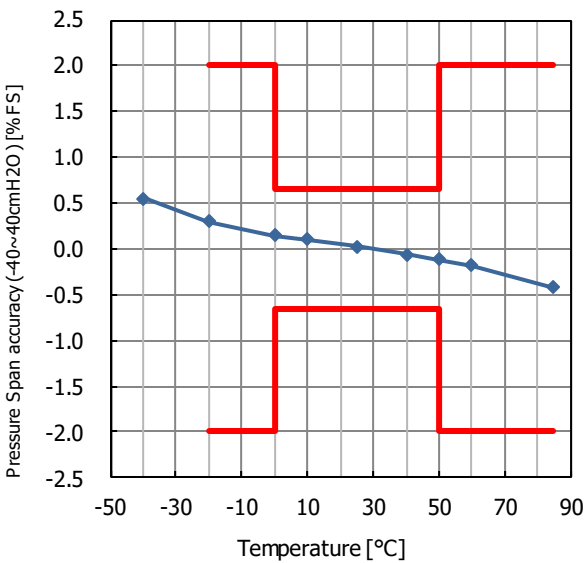
Fig. 20.6 Pressure Span accuracy P_{Sacc} temperature characteristic
