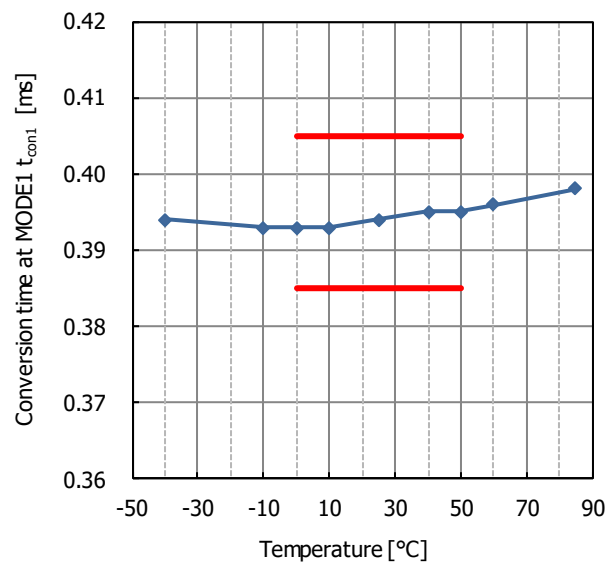
Fig. 19.5 Conversion time at MODE 1 temperature characteristic
