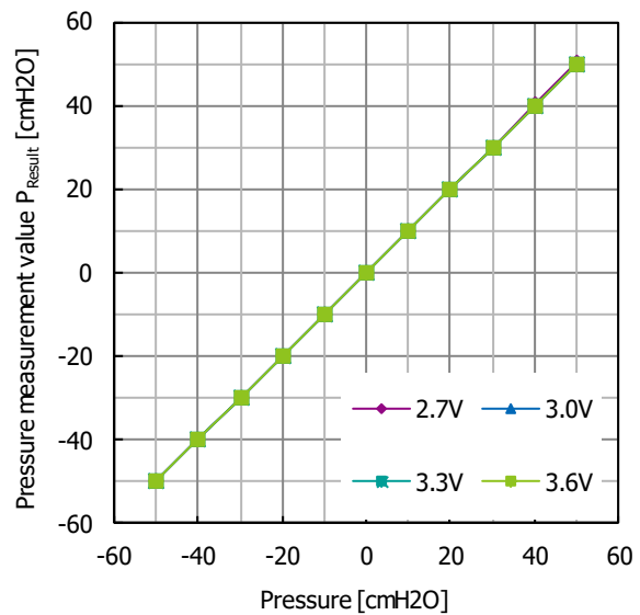
Fig. 20.2 Pressure measurement value P_{Result} supply voltage characteristic
