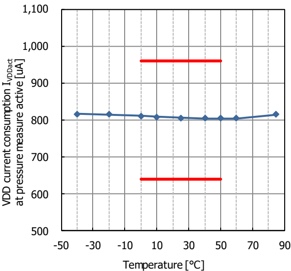
Fig. 19.1 VDD current consumption I_{VDDact} at pressure measure active temperature characteristic
