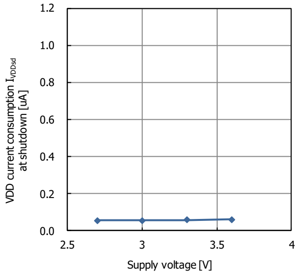
Fig. 19.4 VDD current consumption I_{VDDsd} at shutdown supply voltage characteristic
