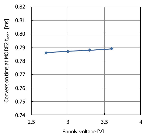
Fig. 19.8 Conversion time at MODE 2 supply voltage characteristic
