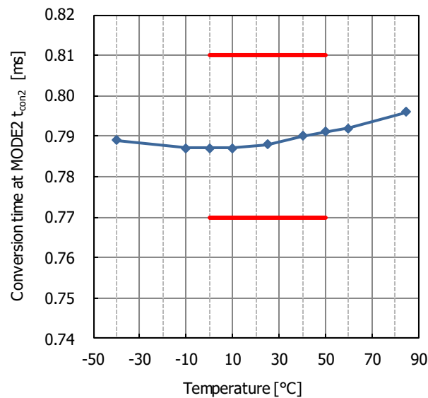
Fig. 19.7 Conversion time at MODE 2 temperature characteristic
