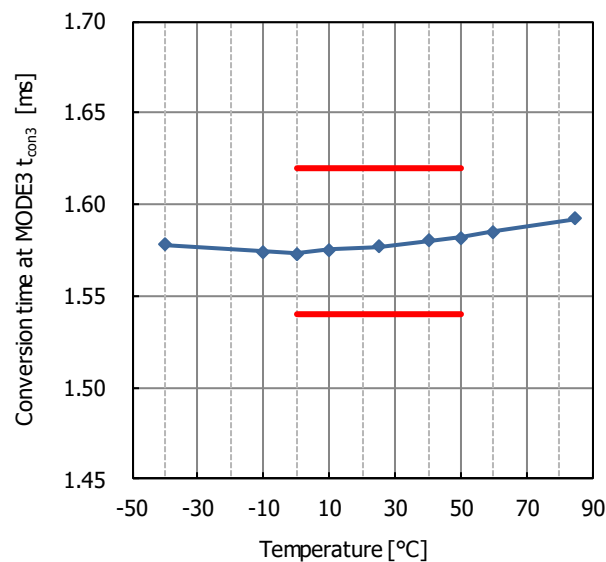
Fig. 19.9 Conversion time at MODE 3 temperature characteristic
