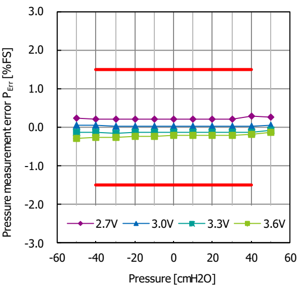
Fig. 20.5 Pressure measurement error P_{Err} supply voltage characteristic
