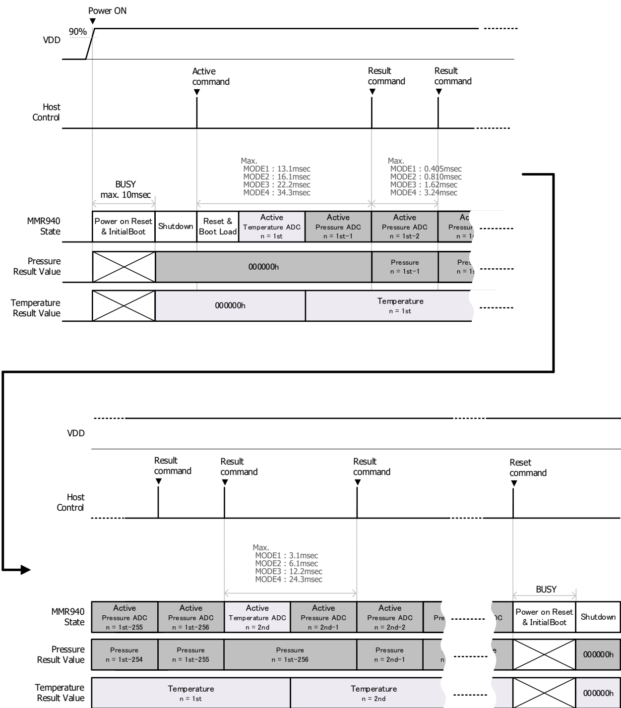
Fig. 9 Timing Chart
