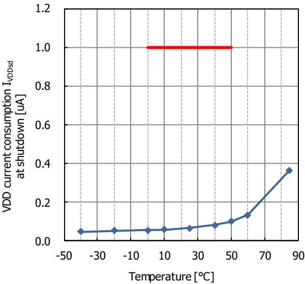
Fig. 19.3 VDD current consumption I_{VDDsd} at shutdown temperature characteristic
