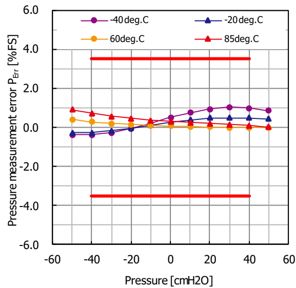
Fig. 20.4 Pressure measurement error P_{Err} temperature characteristic -40~85deg.C
