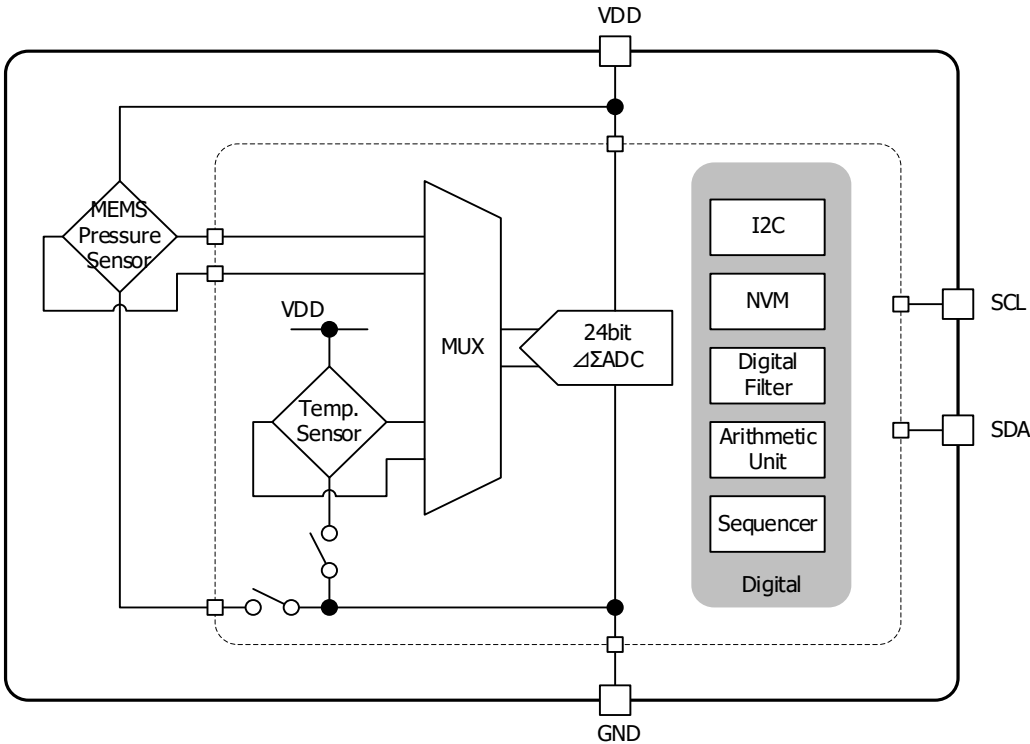
Fig. 1 Block diagram
