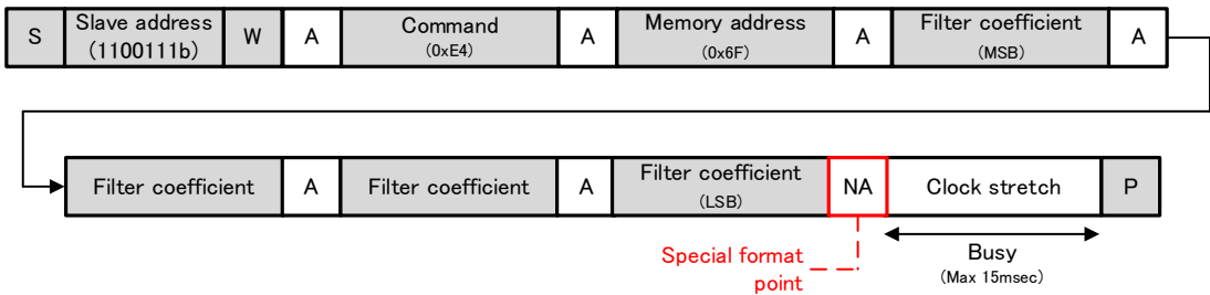
Fig. 15 I2C MACRAM Write format
