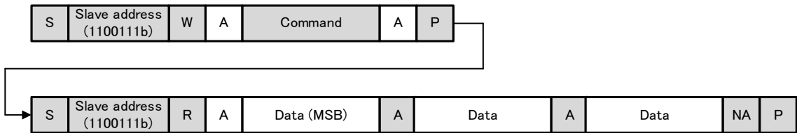
Fig. 14 I2C Combined format
