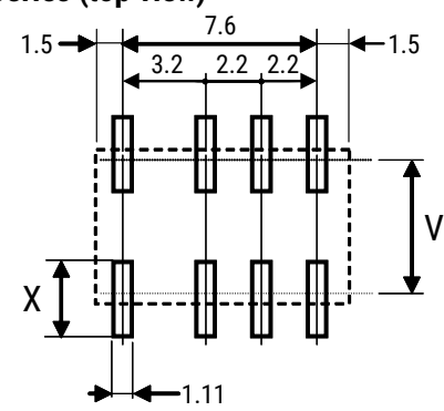
UB2 Series (top view)
