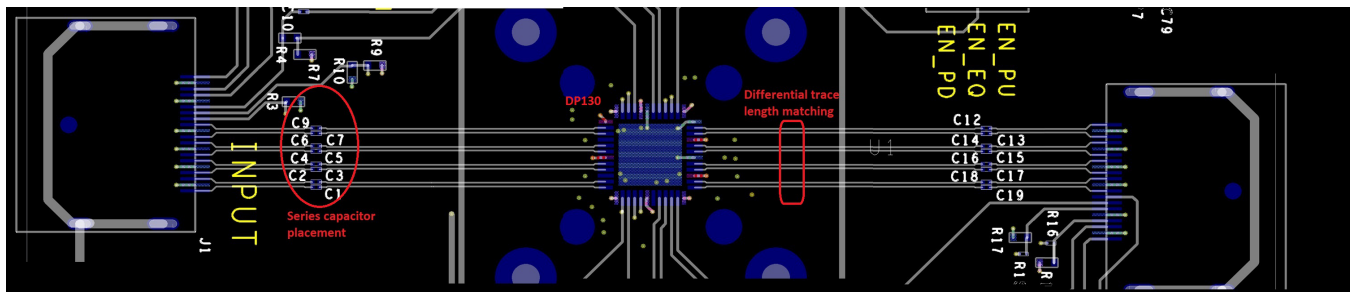
Figure 38. Layout Example
