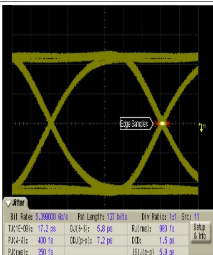
Figure 30. Eye Diagram (EQ = 10 dB)
