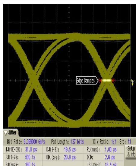
Figure 27. Eye Diagram (EQ = 3.5 dB)
