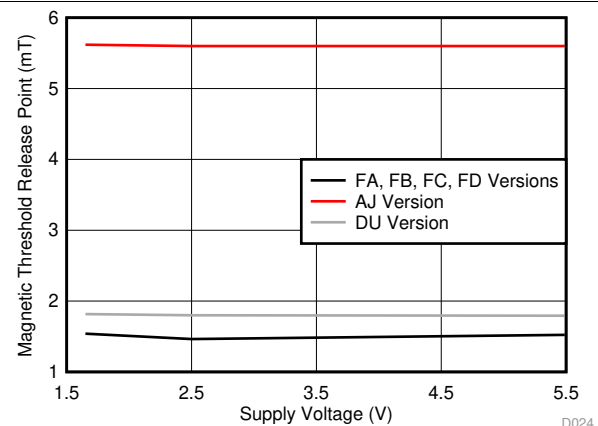
Figure 6. |B_{RP}| vs V_{CC}
