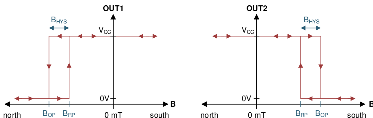
Figure 17. Unipolar Functionality
