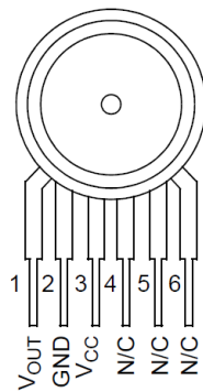
Pinout
