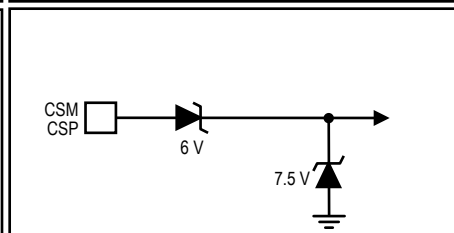
Figure 27h: Current Sense Amp Inputs
