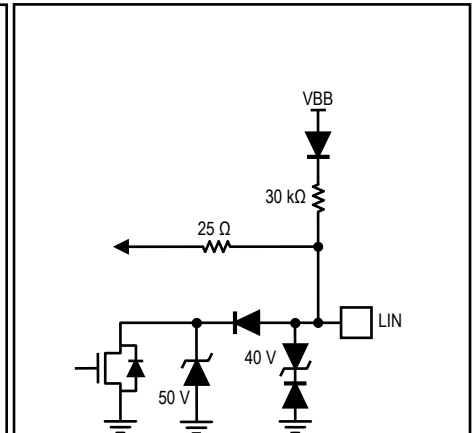
Figure 27c: LIN Bus I/O
