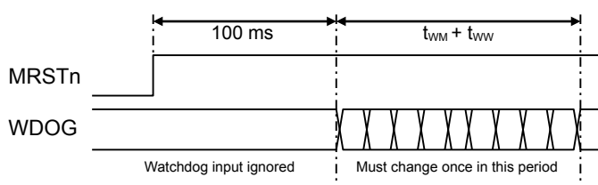
Figure 11e: Timing After Reset
