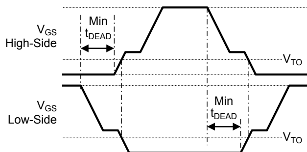
Figure 15: Minimum Dead Time
