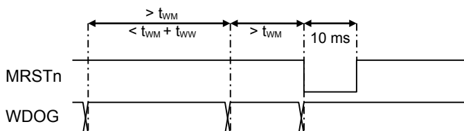
Figure 11d: Reset After Early Watchdog Edge
