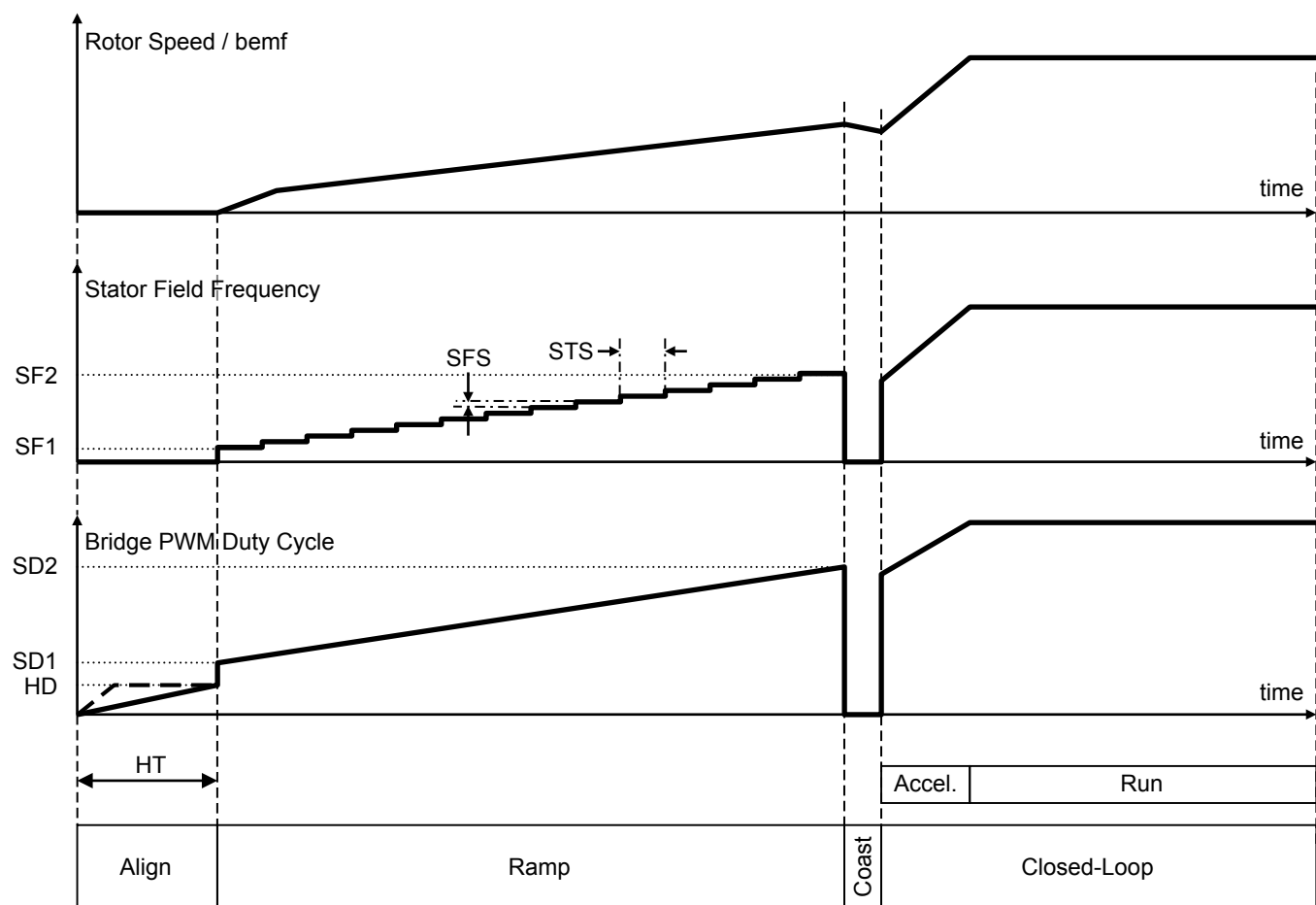
Figure 17: Sensorless Start Sequence
