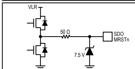
Figure 27g: Logic Output
