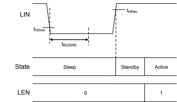
Figure 13a: LIN Wake Sequence and Timing
