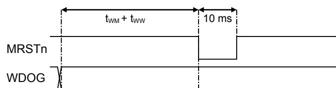
Figure 11c: Reset After Missing Watchdog Edge
