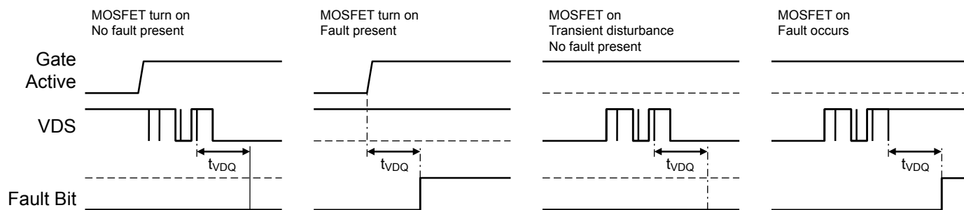
Figure 5b: VDS Fault Detection - Debounce Mode Timing (VDQ = 0)
