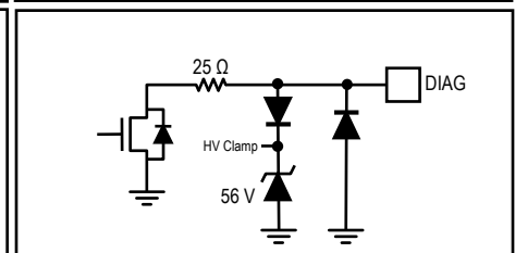
Figure 27i: HV Compliant Output
