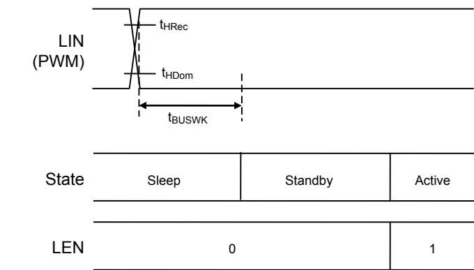
Figure 13b: PWM Wake Sequence and Timing
