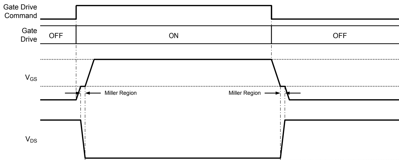
Figure 14b: Off-to-On and On-to-Off Transitions with Gate Drive Control Disabled
