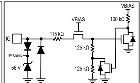
Figure 27f: HV Compliant Logic Inputs
