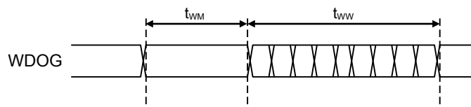
Figure 11a: Watchdog Timing Requirements
