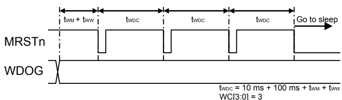
Figure 11f: Sleep After Fail Cycle Count
