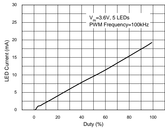
PWM Dimming
