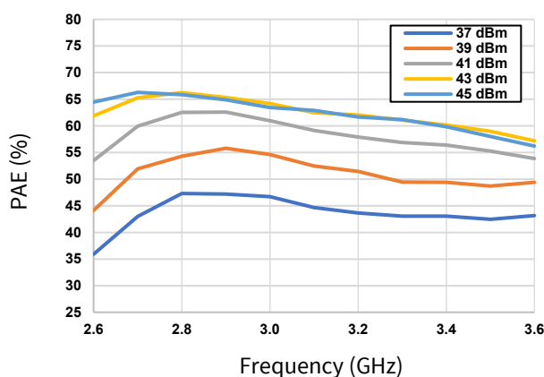
Figure 4. Power Added Efficiency vs. Frequency as a Function of Input Power
