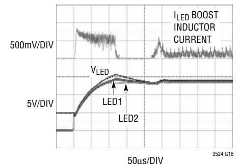
LED Initial Start-Up Waveforms
