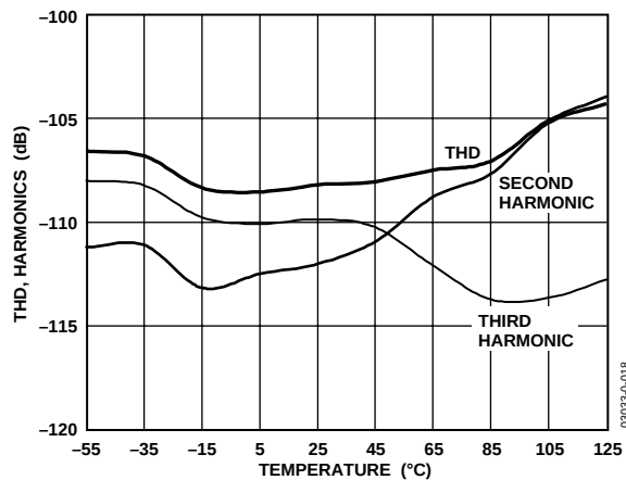
Figure 18. THD and Harmonics vs. Temperature
