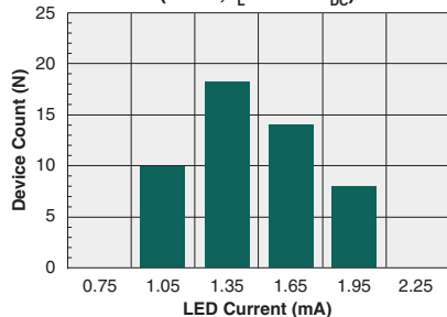
Typical I_F for Switch Operation (N=50, I_L=150\text{mA}_{DC} )
