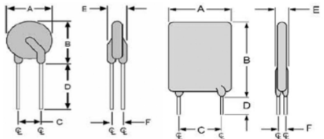
Fig.3 Lead Size : 20AWG Φ0.81 mm Diameter
